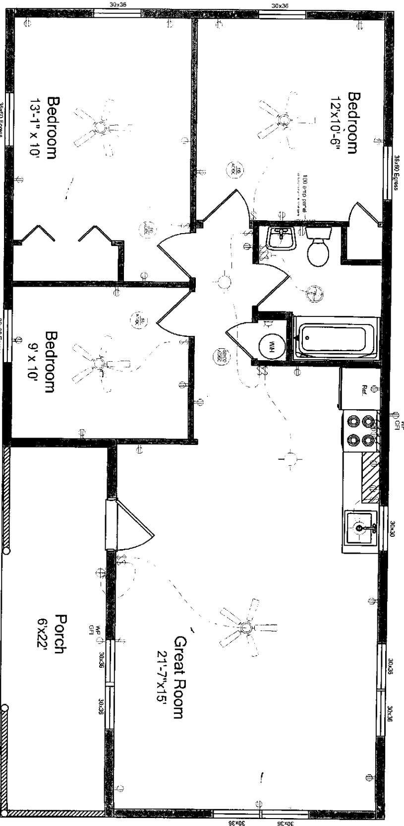
Plan 22CC603-H 22'x48' with 6' x 22' porch included
