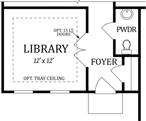
PARTIAL FIRST FLOOR PLAN W/ CHOICE - LIBRARY
