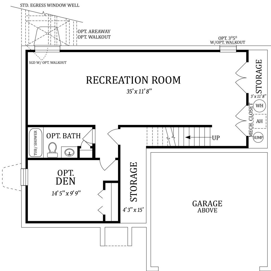
OPT. FINISHED LOWER LEVEL
